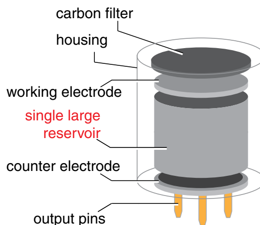
Figure 1: Conventional cell technology
