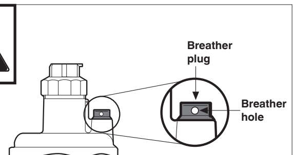
Never close Breather hole!
