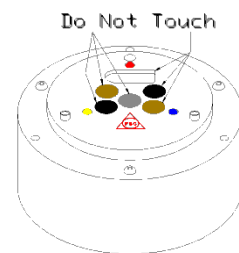
Detector Module "puck" Figure 2-4
