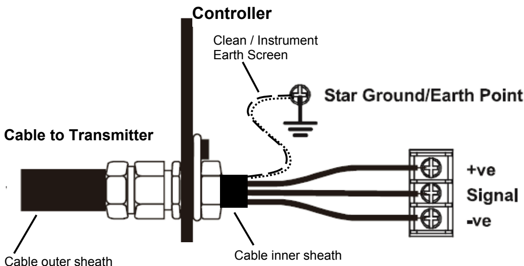
Diagram 10: Controller Grounding
