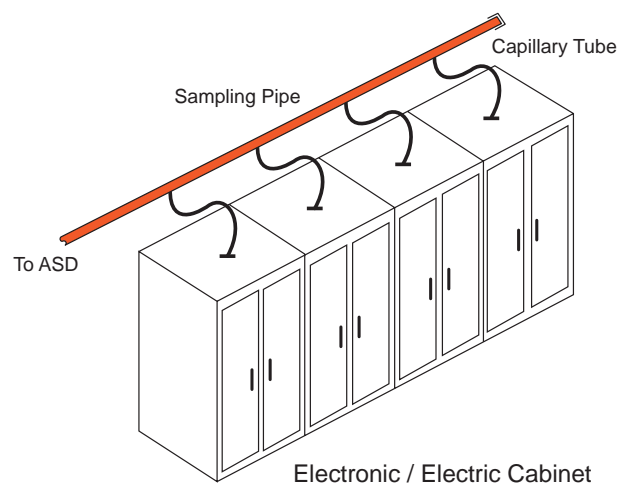
Figure 7. Sampling electronic/electrical cabinets utilising capillary sampling points
