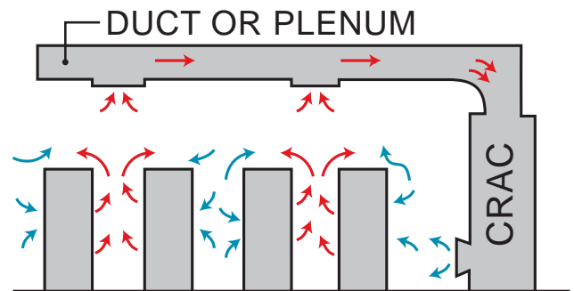
A flooded supply with a targeted air return scheme. Hot air can mix with cold air supply.
