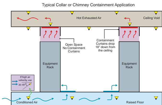
Typical collar or chimney containment application. Shown are typical air sample point locations: 1. Under raised floor (code/insurer requirement or combustibles present). Sampling points located in air flow. If high air velocities orient hole 20–45° downward facing into airflow. (See BS 6266 for hole spacing adjustments) 2. Above ceiling return air plenum (code/insurer requirement or combustibles present). (See BS 6266 for hole spacing adjustments). 3. Below ceiling for general area protection. 4. Air transfer grills at top of hot collar or chimney
