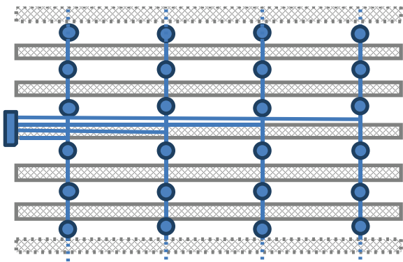
Figure 15 .- Standard Rectangular Layout
