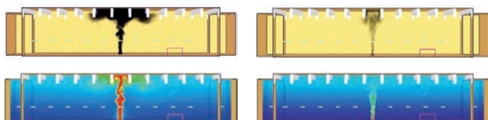
Figure 4 – Fire development in a near constant temperature environment
