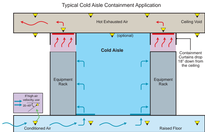
Typical cold aisle containment application. Shown are typical air sample point locations: 1. Under raised floor (code/insurer requirement or combustibles present). Sampling points located in air flow. If high air velocities orient hole 20–45° downward facing into airflow. (See BS 6266 for hole spacing adjustments) 2. Above ceiling return air plenum (code/insurer requirement or combustibles present). (See BS 6266 for hole spacing adjustments). 3. Below ceiling for general area protection. Air flow in cold aisle is not targeted to ceiling consequently, ceiling detection in cold aisle is optional, but may be of value during work operations or for protection against transient fuel loads in the cold aisle. 4. Top of hot aisle air transfer grills
