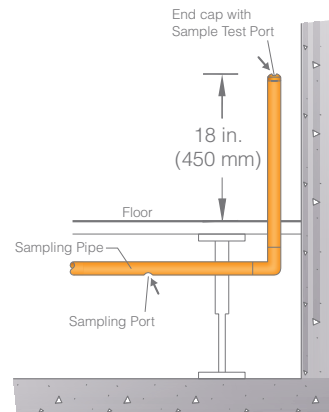
Figure 11. 3-Test sample point for void space or sub-floor
