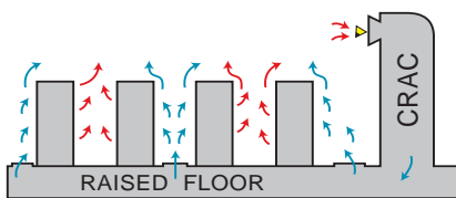
A targeted air supply with a flooded return air system. Cold supply air mixes with hot return air. Install air sampling ports at main return into HVAC/CRAC unit.
