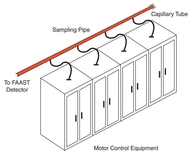
Figure 5. Sampling motor control units utilising capillary sampling points
