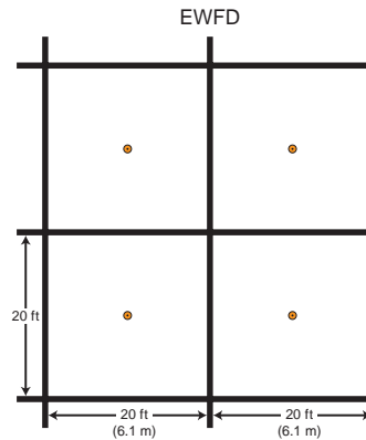
Example arrangement of sampling ports located to meet requirements for EWFD structural bays of 400 ft 2 (37.2 m 2 )
