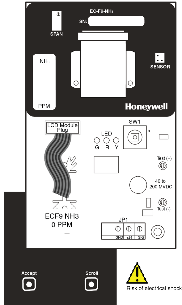
Figure 7. LCD Module
