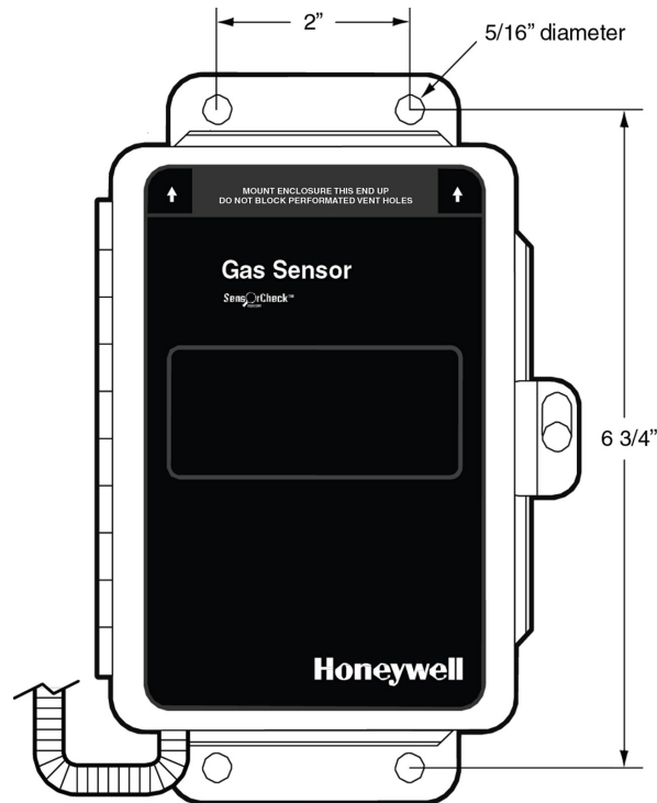
Figure 1. Mounting Dimensions
