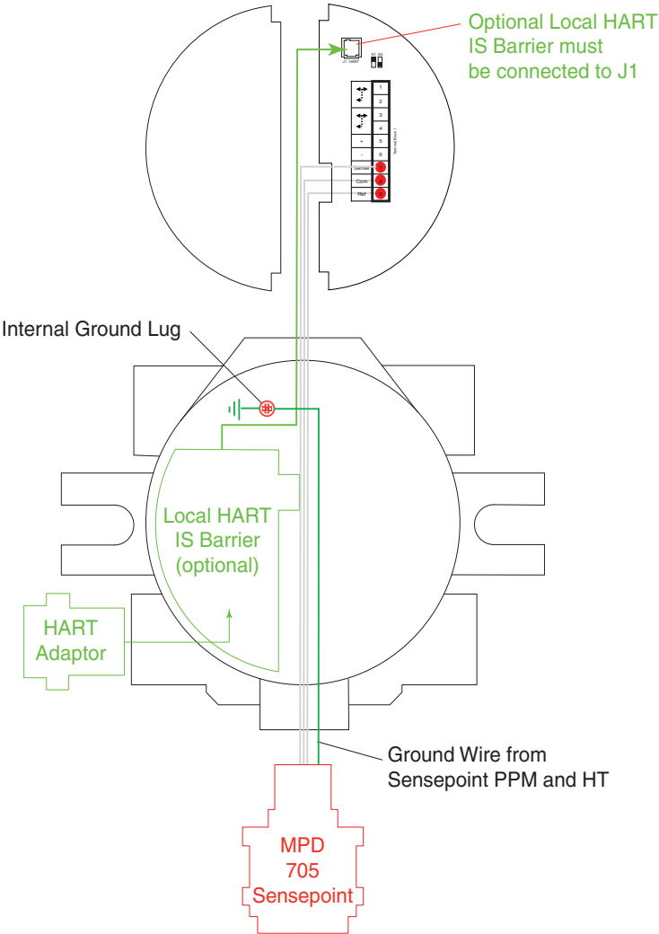
Figure 46. mV Personality Wiring
