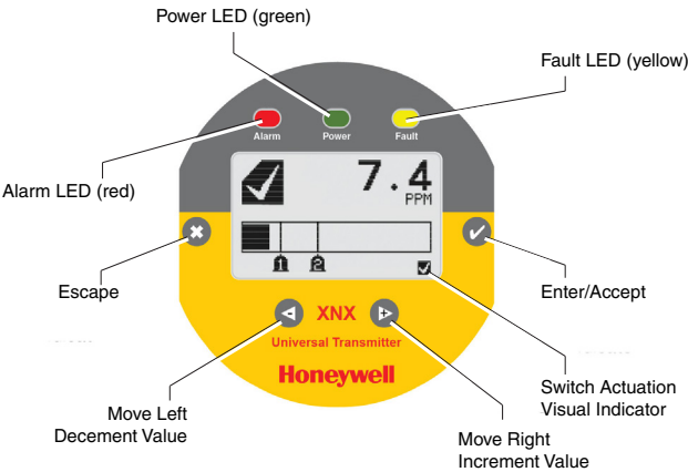
Figure 11. Front panel display of the XNX transmitter
