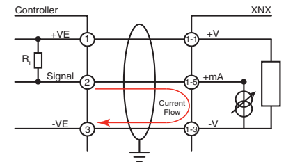
Figure 36. Sink wiring for XNX
