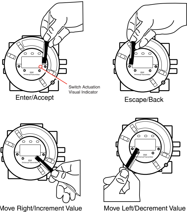
Figure 9. Using the magnetic wand
