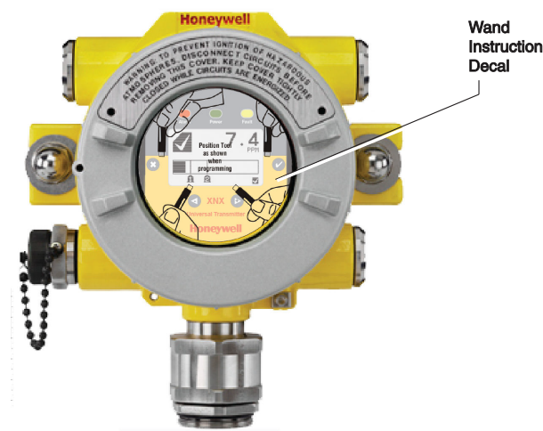
Figure 10. Operation decal
