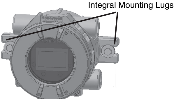
Figure 26. XNX Universal Transmitter mounting lugs
