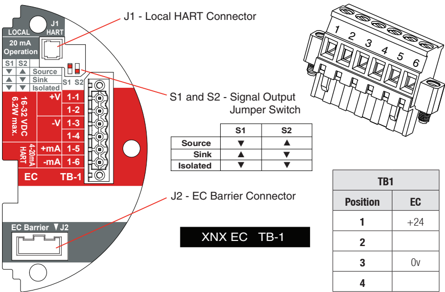
Figure 41. XNX EC Personality Board Terminal Blocks and Jumper Switches and Terminal Block Assignments
