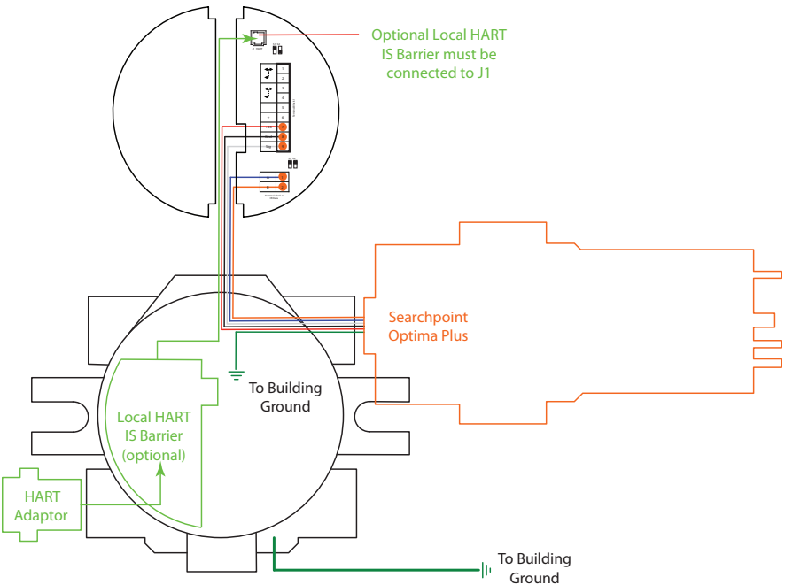
Figure 51. XNX IR Personality Board Terminal Blocks, Jumper Switches and Wiring Guide
