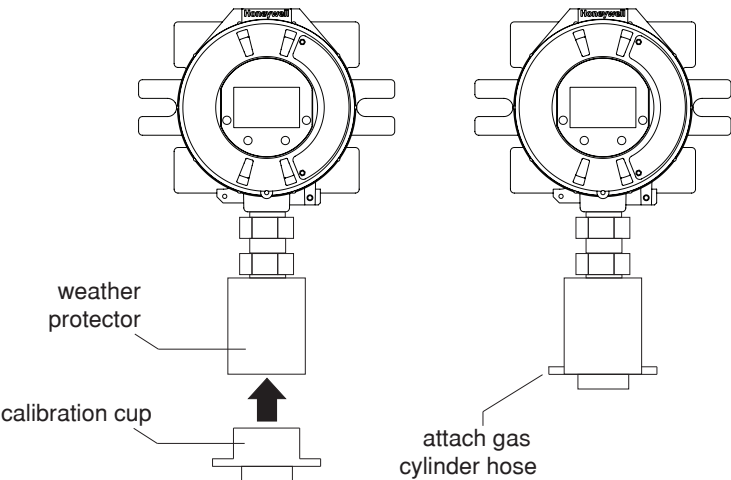
Figure 203. Attaching the Calibration Cup
