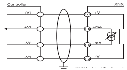
Figure 38. Isolated wiring for XNX
