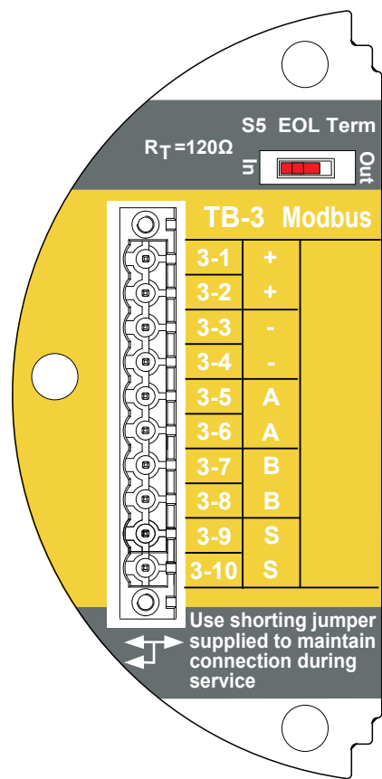
Figure 248. Modbus connections
