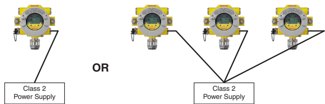
Figure 32. Single transmitter distances
