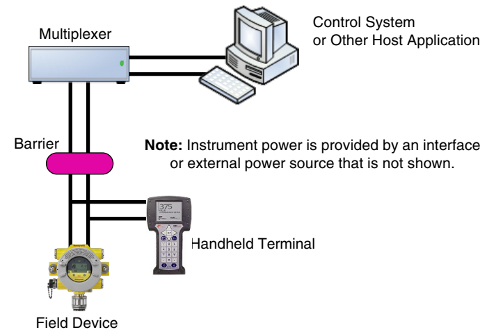
Figure 57. Point-to-Point Mode of Operation
