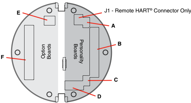
Figure 35. XNX Personality Board Terminal Block Legend
