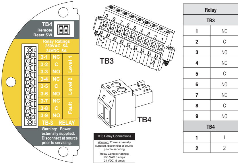
Figure 59. XNX Relay Option Board Terminal Blocks
