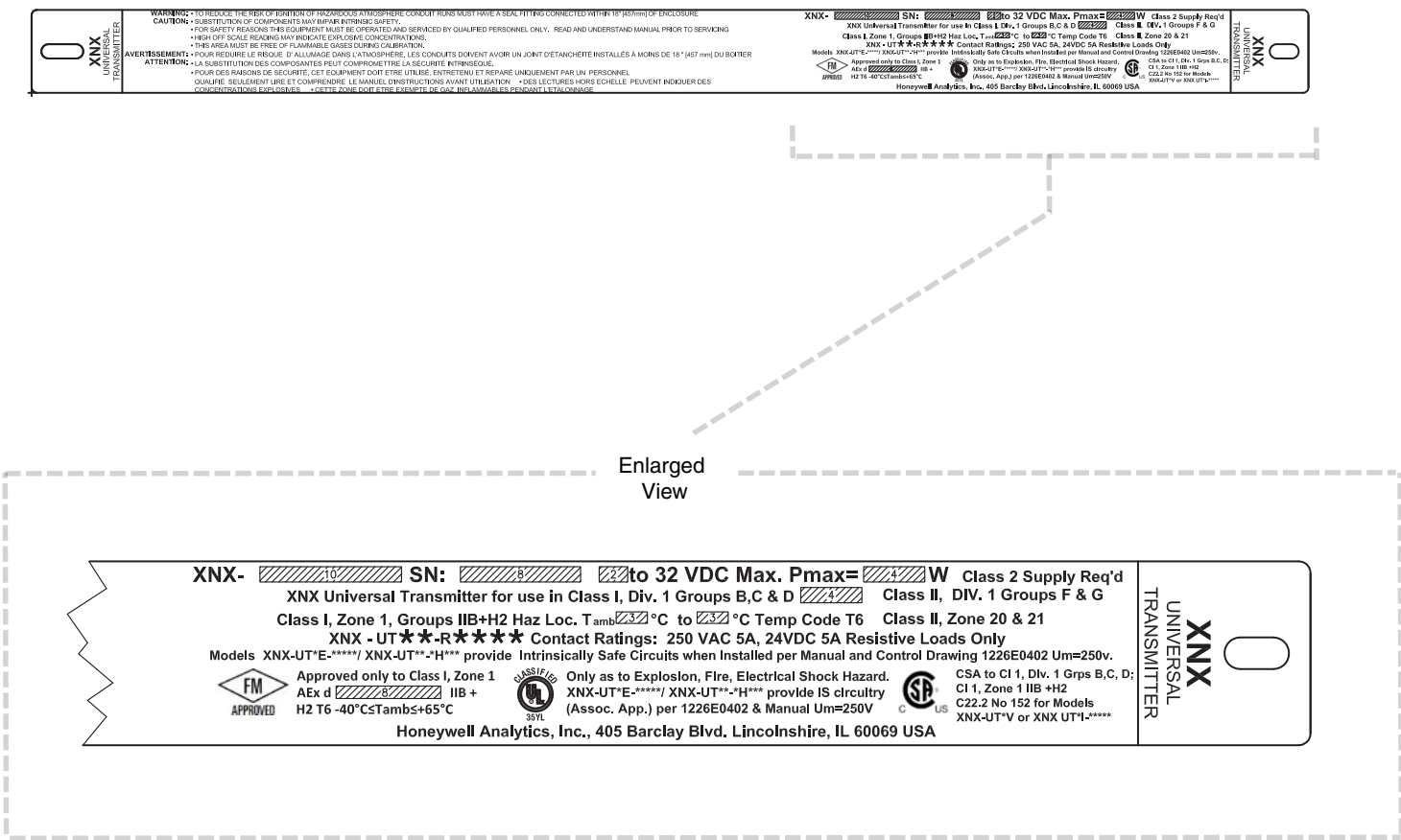
Figure 230. XNX-UT**-***** Configuration
