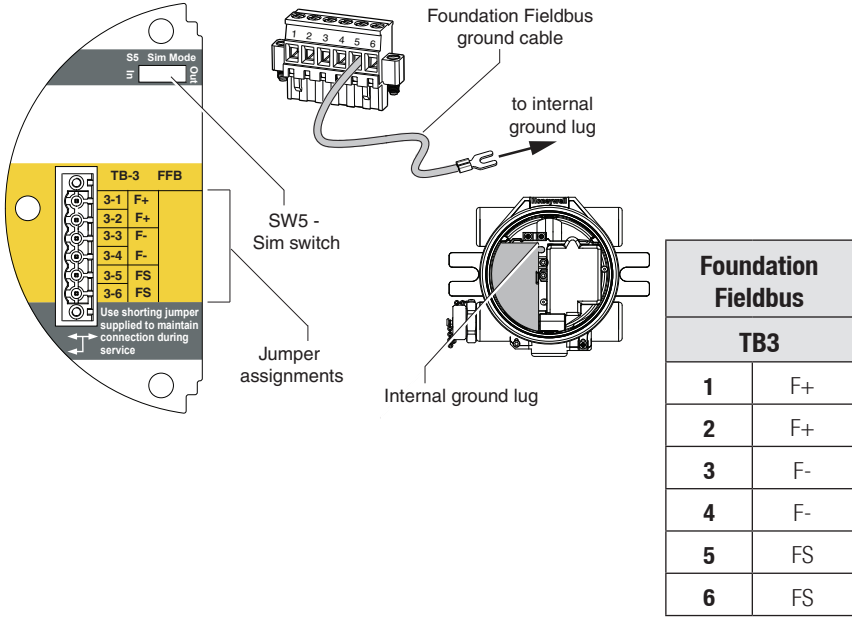
Figure 61. Foundation Fieldbus Option Board, Terminal Block, Jumper Switch
