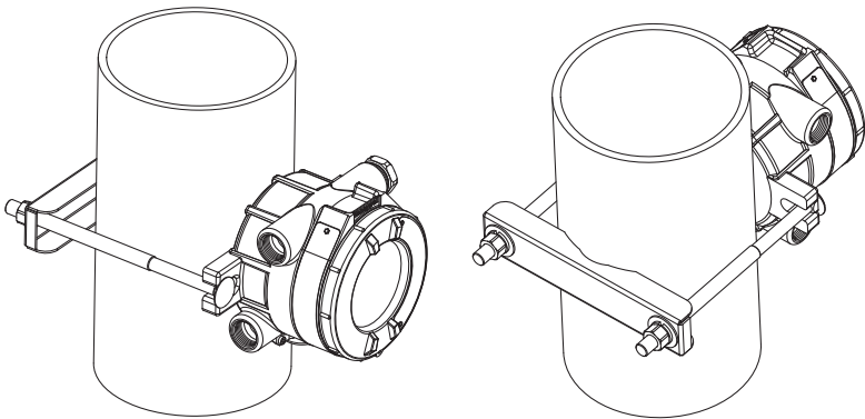
Figure 8. Pipe-mounted XNX Transmitters
