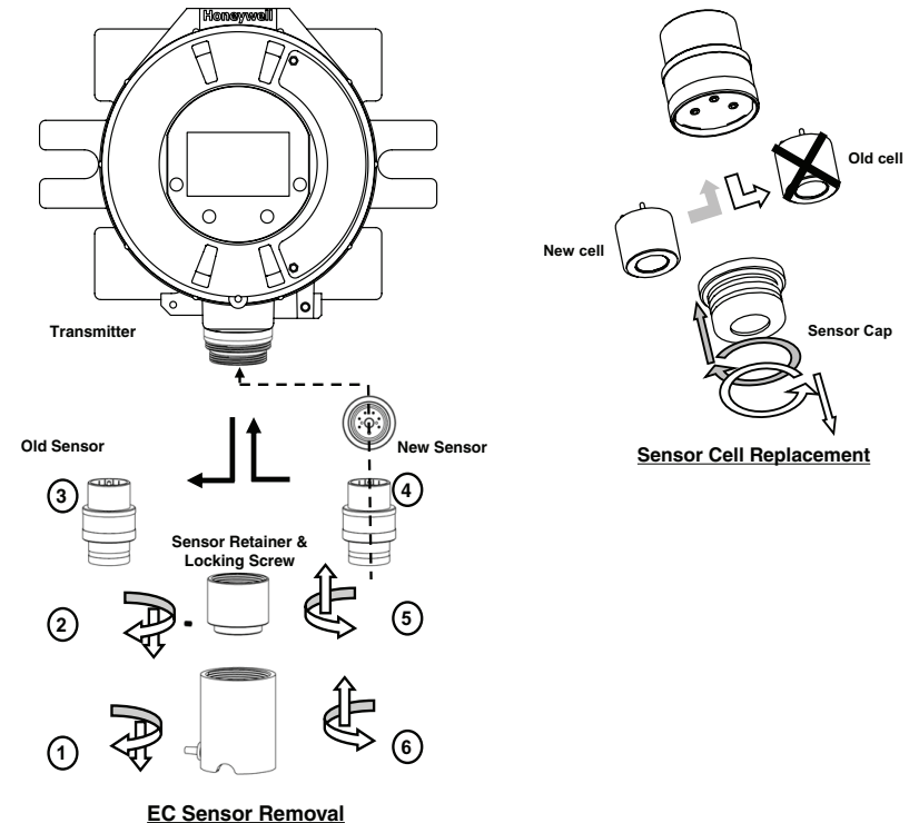
Figure 228. XXN EC Sensor Cell Replacement
