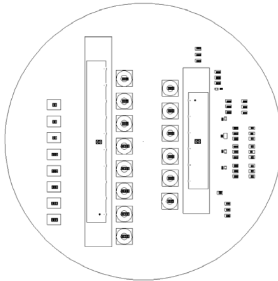
Figure 2-12 Terminals
